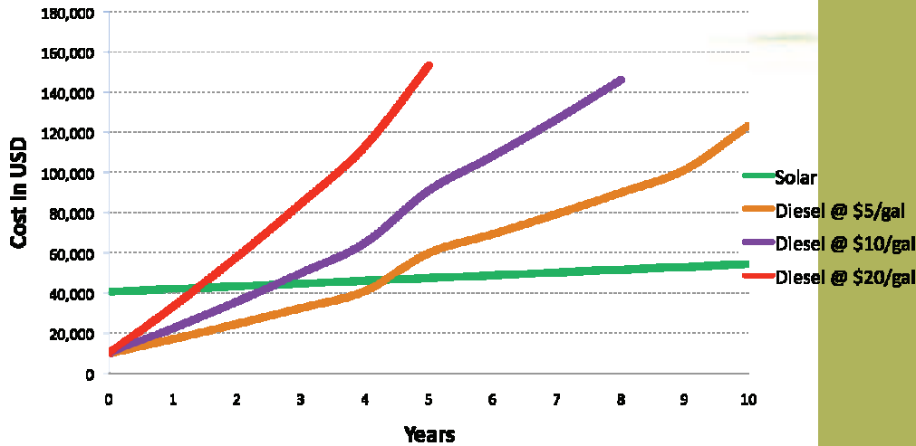
Solar v. Diesel Generator Lifetime Costs (8-12 Hours/Day Operation)
